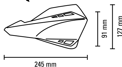
SABRE with Wind Deflectors fitted
